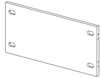
H Bottom Back Rail x1 Barra trasero inferior #42629
