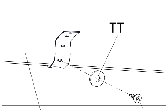
Bottom Back Rail BarraTraseroInferior
