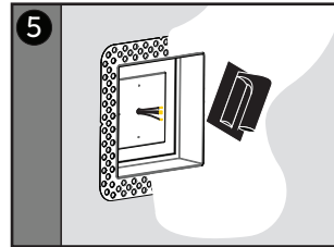
5 Use drywall compound mud to cover flange. Once dry, sand. Repeat as needed.
