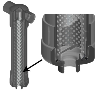
Socket/Spigot
