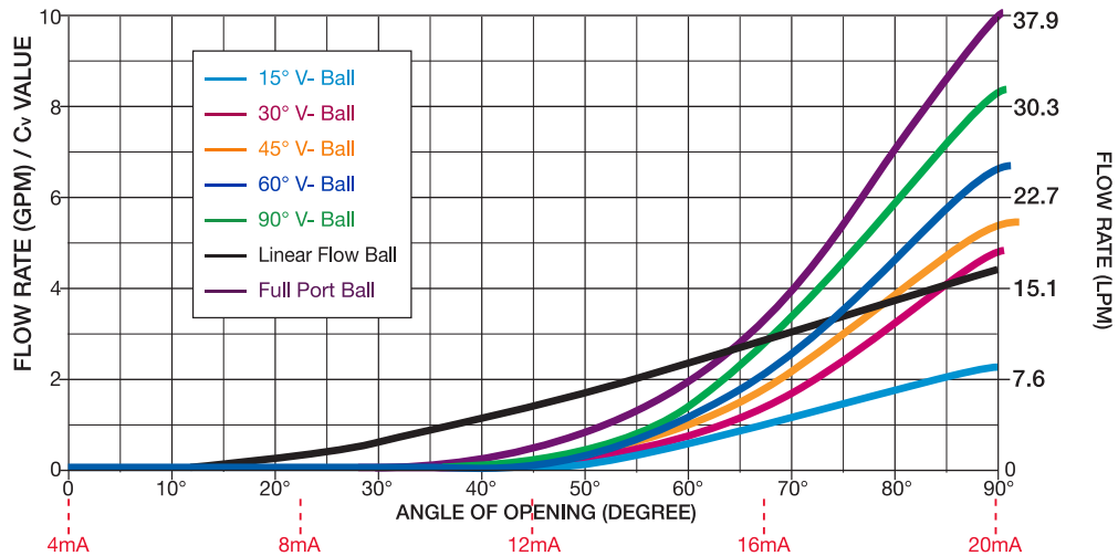
1/2" Valve
