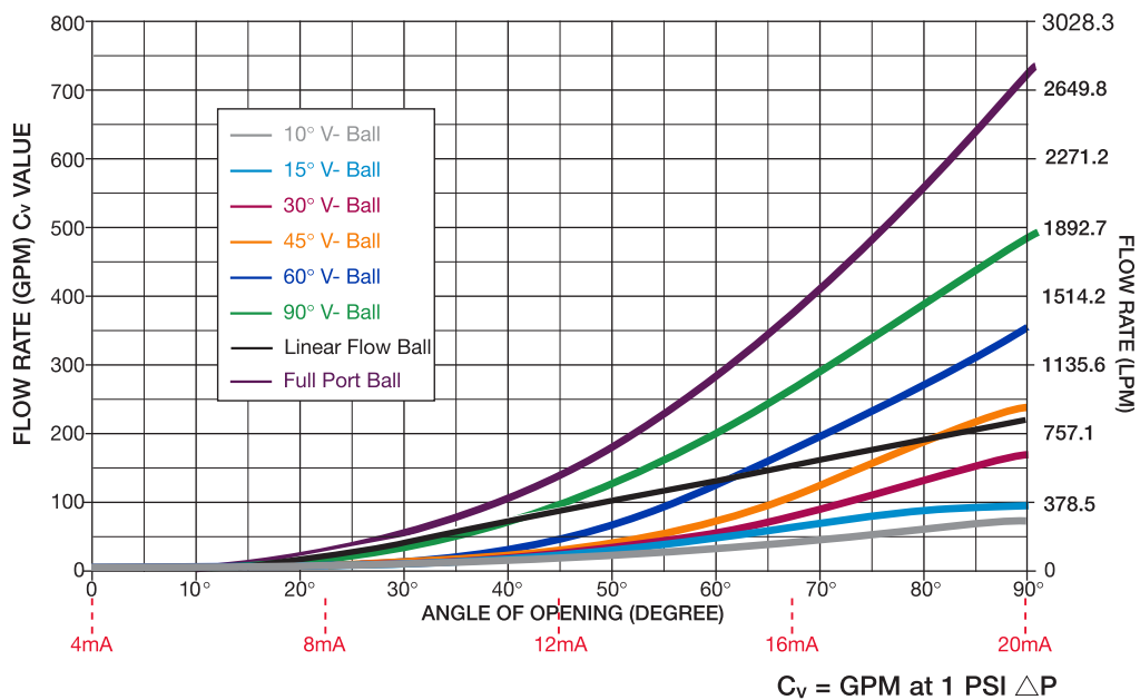
4" Valve
