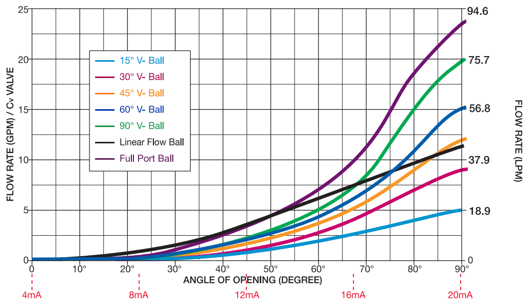
3/4" Valve
