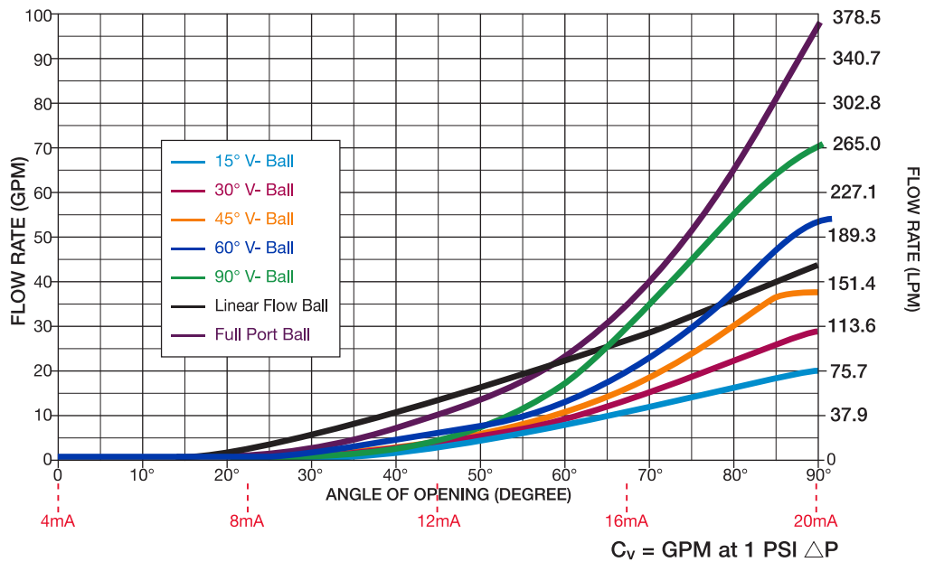
1 1/2" Valve
