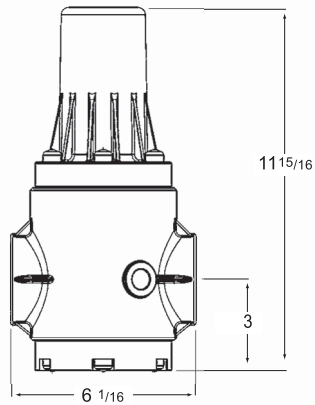
1 1/2" Socket or Threaded
