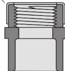
Hexagonal Wrench Flats Easy Threaded Joint Make-up
