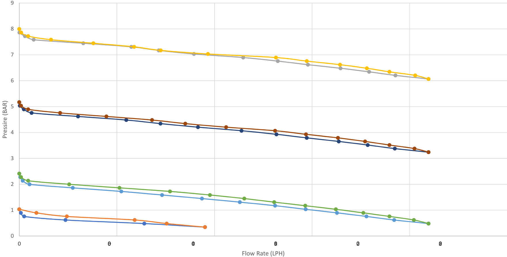
PRHM 150 Flow Chart Metric
