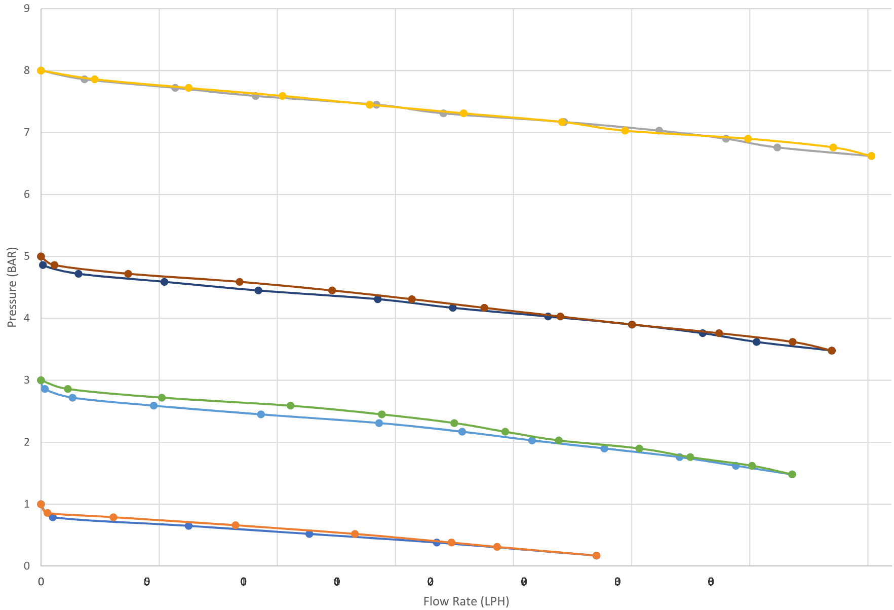
PRHM050EP-PV Flow Rate Metric
