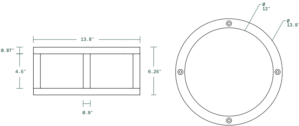
Stand Dimensions [NOT TO SCALE]
