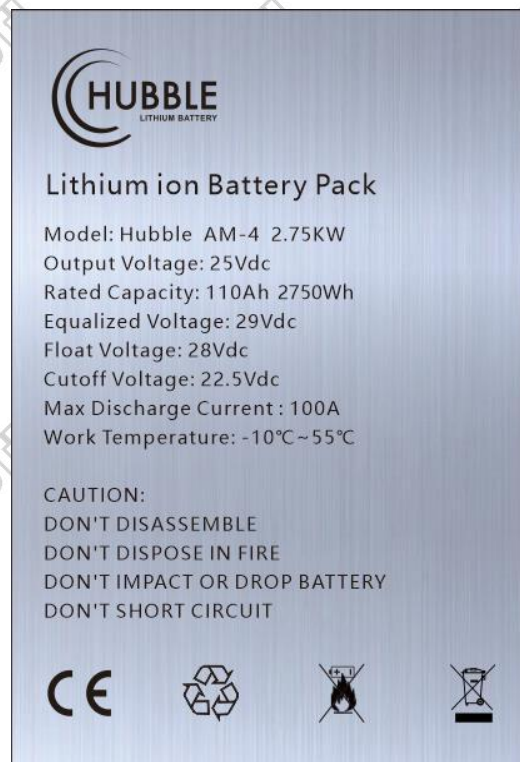
Figure 4 Battery Label (电池标签)
