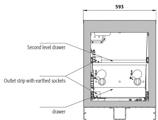
Sectional view
