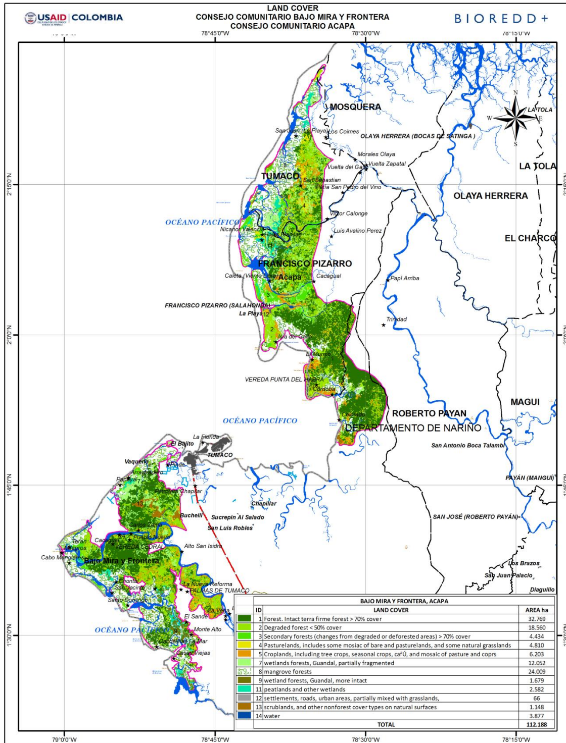
Figure 8. Vegetation cover.
