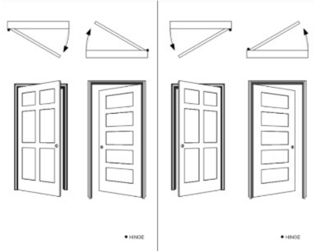
LEFT HAND SWING
