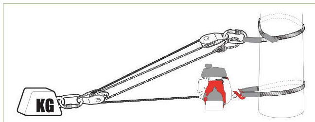
MEKANISK FORDEL X 4
