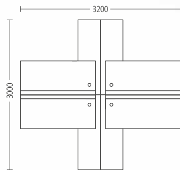
WORKSTATION 3200W x 3000D x 750H (mm)
