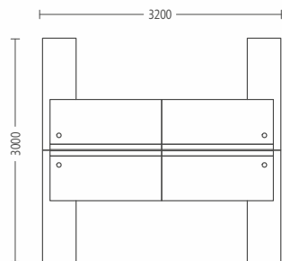
WORKSTATION 3200W x 3000D x 750H/1200H (mm)
