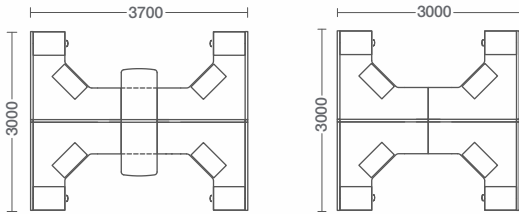
WORKSTATION WITH & WITHOUT D CABINET 3700W x 3000D x 1200H (mm) / 3000W x 3000D x 1200H (mm)
