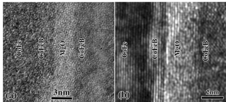
Fig. 5: Cross sectional images of a magnetic tunneling junction. Materials after annealing (b) are much less disordered structurally than before annealing (a).
