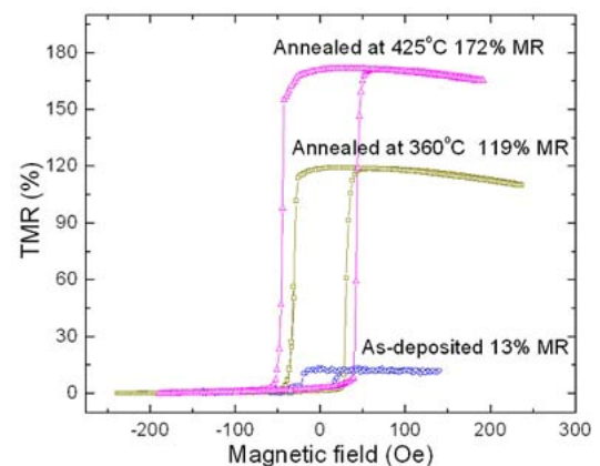
Fig. 7: Magnetic thermal annealing can reorient and strengthen the easy axis of a magnetic thin film, allowing for much higher magnetization in a magnetic field
