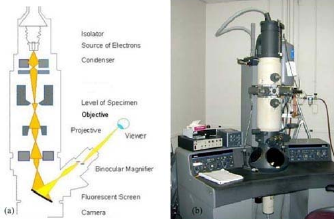
Fig. 4: Schematic drawing of a transmission electron microscope (a) and a photograph of a Phillips 420 TEM
