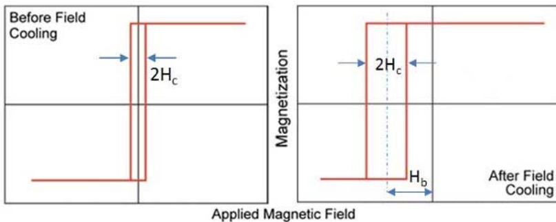
Fig. 1: Hysteresis loops demonstrating the appearance of exchange bias after magnetic thermal annealing
