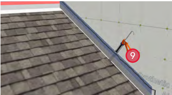
9. Install sealant along the exposed waterproof roof deck membrane. Extend the sealant down to the extent of overlap from the above layer of sheathing membrane to maintain air barrier continuity.
