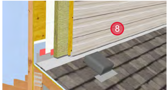
8. Install cladding.
