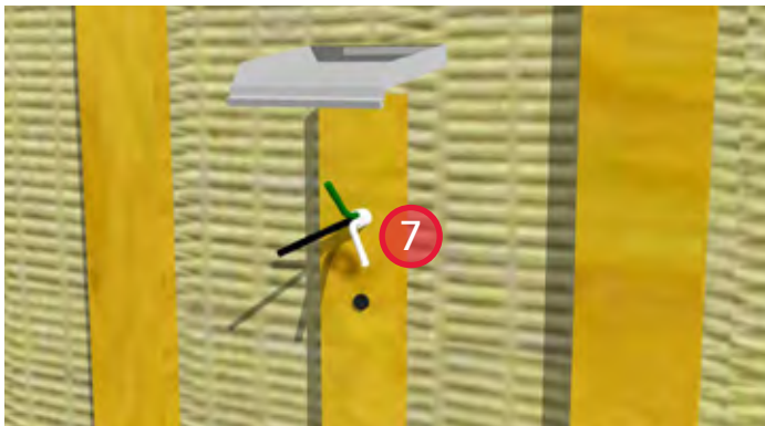
7. Install ROCKWOOL COMFORTBOARD™ 80 and strapping. Provide bugscreens at the top and bottom of the strapping.
