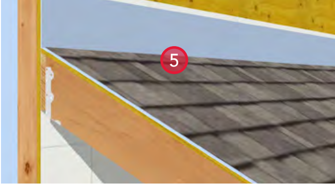
5. Install shingles.
