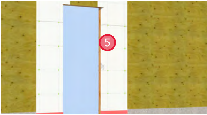
5. Install sheathing membrane at the jambs and seal the leading edge with sheathing tape. Extend the membrane into the rough opening.
