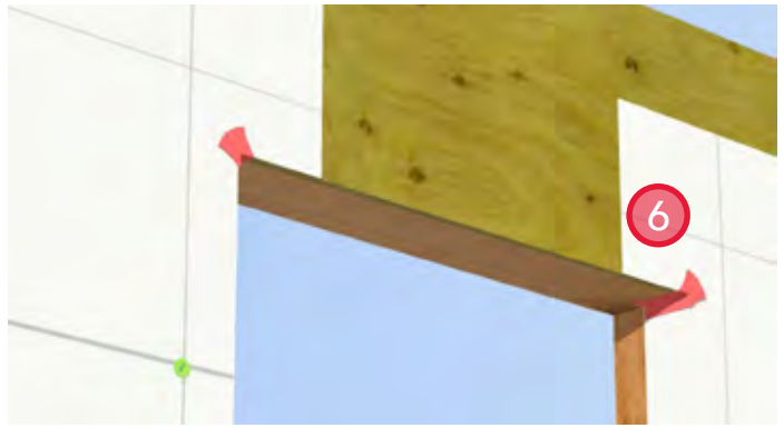
6. Install gussets constructed from sheathing tape at the upper corners of the rough opening.
