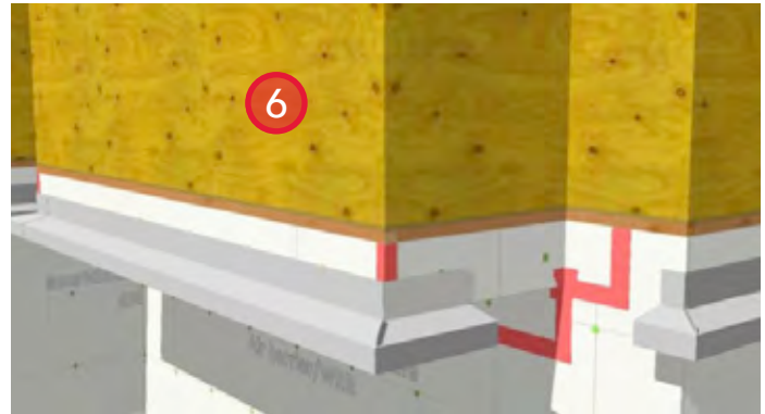
6. Install prefinished metal flashing around the base of the cantilevered section.
