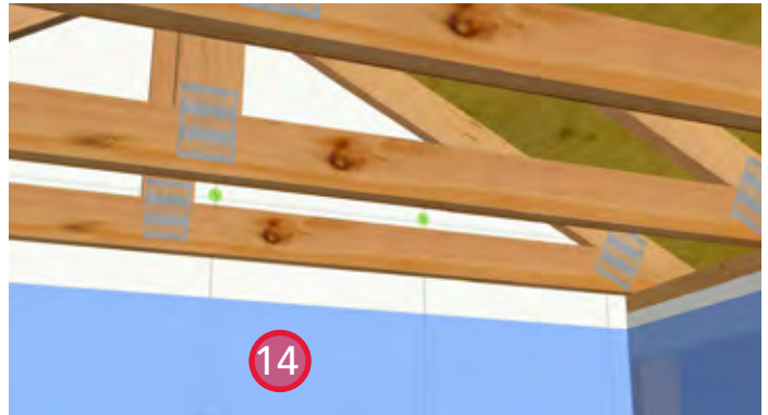
14. Install poly on the walls and fasten to the sheathing membrane with staples.
