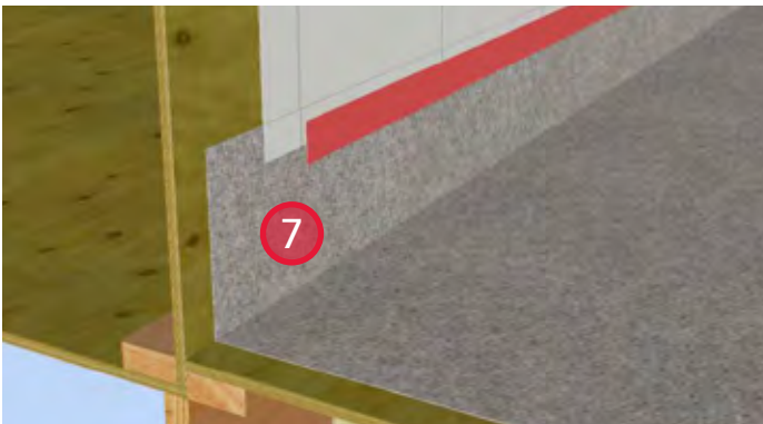
7. Install sheathing membrane and seal the leading edge to the balcony membrane with sheathing tape to maintain air barrier continuity.
