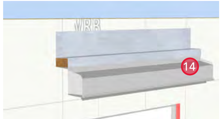
14. Install self-adhered membrane over the wood blocking. Extend the membrane onto the adjacent wall and the prefinished metal flashing.
