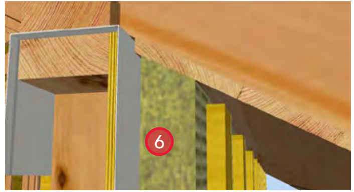
6. Install ROCKWOOL COMFORTBOARD™ 80 and strapping to the exterior of the wall. Provide bugscreens at the top and bottom of the strapping.
