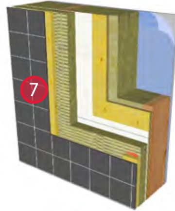
7. Install wire support mesh.
