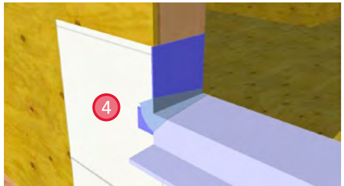
4. Install self-adhered membrane gussets at lower corners.
