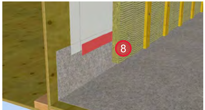
8. Install ROCKWOOL COMFORTBOARD™ 80 insulation and strapping to the exterior of the wall. Provide bugscreens at the top and bottom of the cladding.
