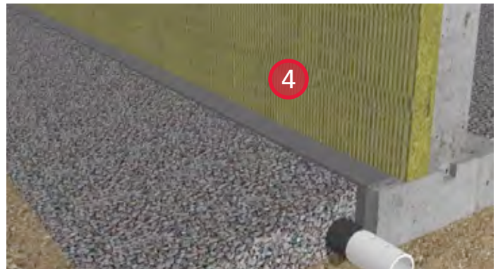
4. Install ROCKWOOL rigid board insulation against foundation wall. Spot adhere the insulation to prevent puncture of the waterproofing membrane.
