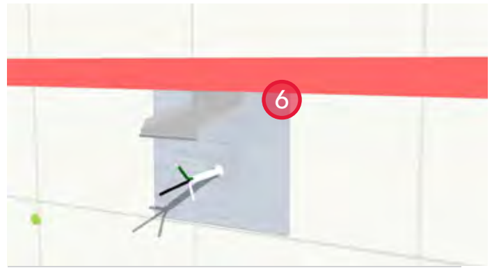
6. Install second layer of sheathing membrane and lap over the metal flashing. Seal the leading edge with sheathing tape to maintain air barrier continuity.
