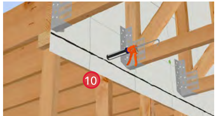
10. Apply a bead of sealant to the exterior of the sheathing membrane to provide for air barrier continuity.
