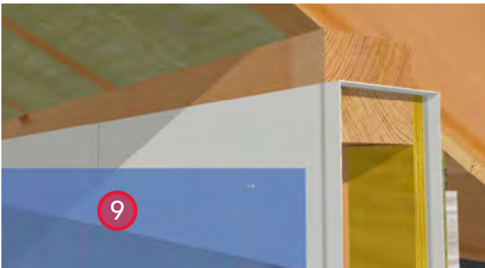
9. Install the poly sheet on the interior face of the wall. Fasten the poly to the sheathing membrane with staples at each stud.
