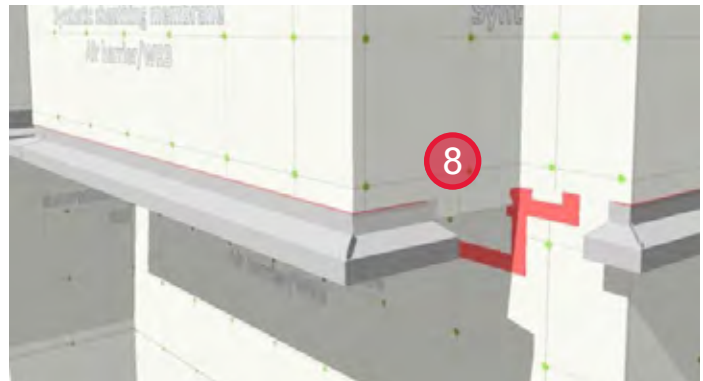
8. Lap sheathing membrane over the flashing.
