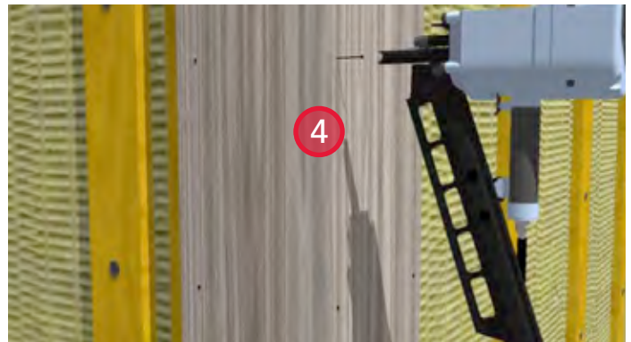
4. The corner trim boards must be nailed together as well as to the strapping to form the corner.
