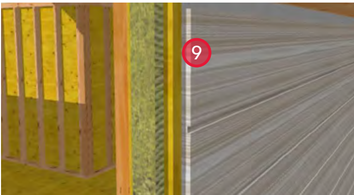
9. Install cladding. Provide venting at the top of the wall to allow for the free movement of air through the wall cavity. It is not recommended to vent the wall cavity into the roof.
