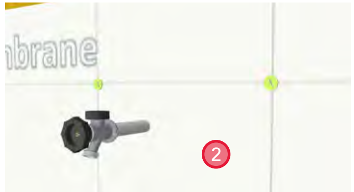
2. Install frost-free hose bib through an appropriately sized penetration.
