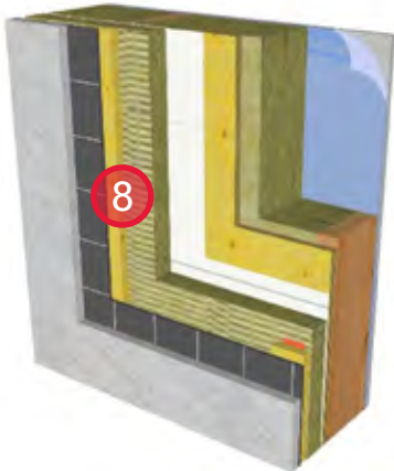
8. Install stucco finish.
