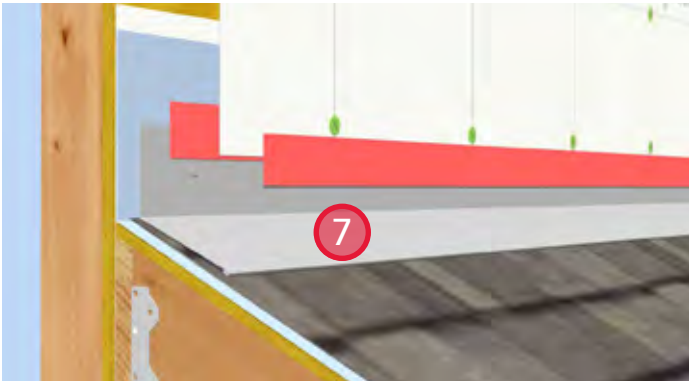
7. Install sheathing membrane. Lap the membrane over the closure flashing and seal the leading edge with sheathing tape to maintain air barrier continuity.
