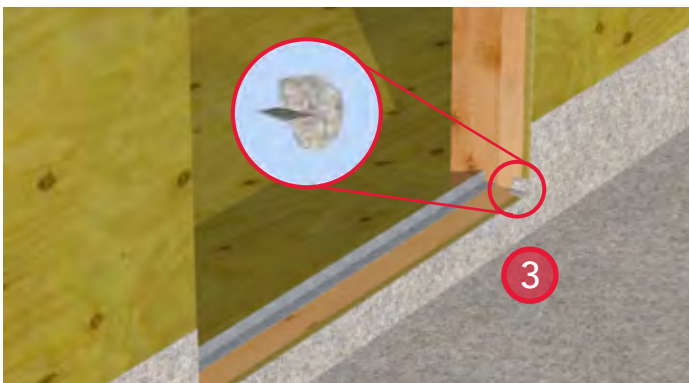
3. Install gussets made from PVC membrane at the corners of the rough opening.
