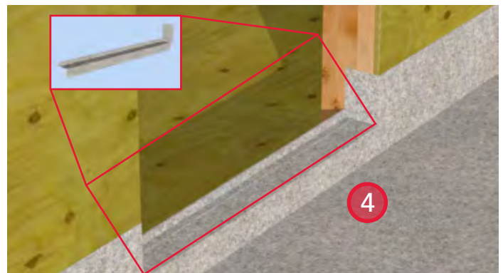
4. Install a sill membrane constructed from PVC membrane. Extend the membrane 2" onto the face of the wall and up the jamb a minimum of 6".
