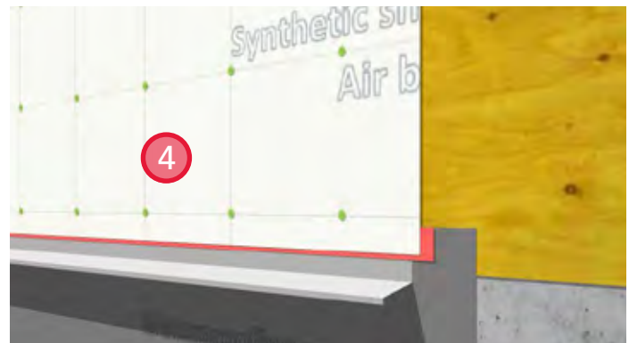
4. Install sheathing membrane and seal leading edge with sheathing tape to complete air barrier continuity. Provide a \frac{3}{4} " vision line on the flashing backleg.
