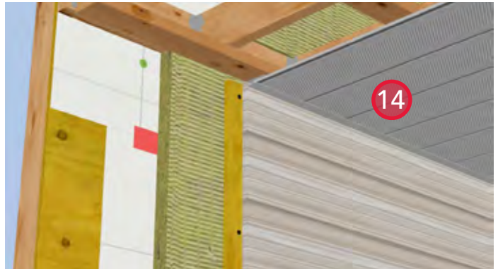
14. Install vented soffit material.
