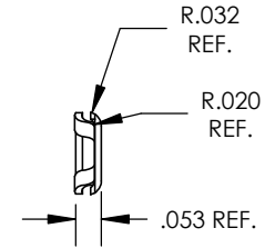
DETAIL D SCALE 2 : 1
