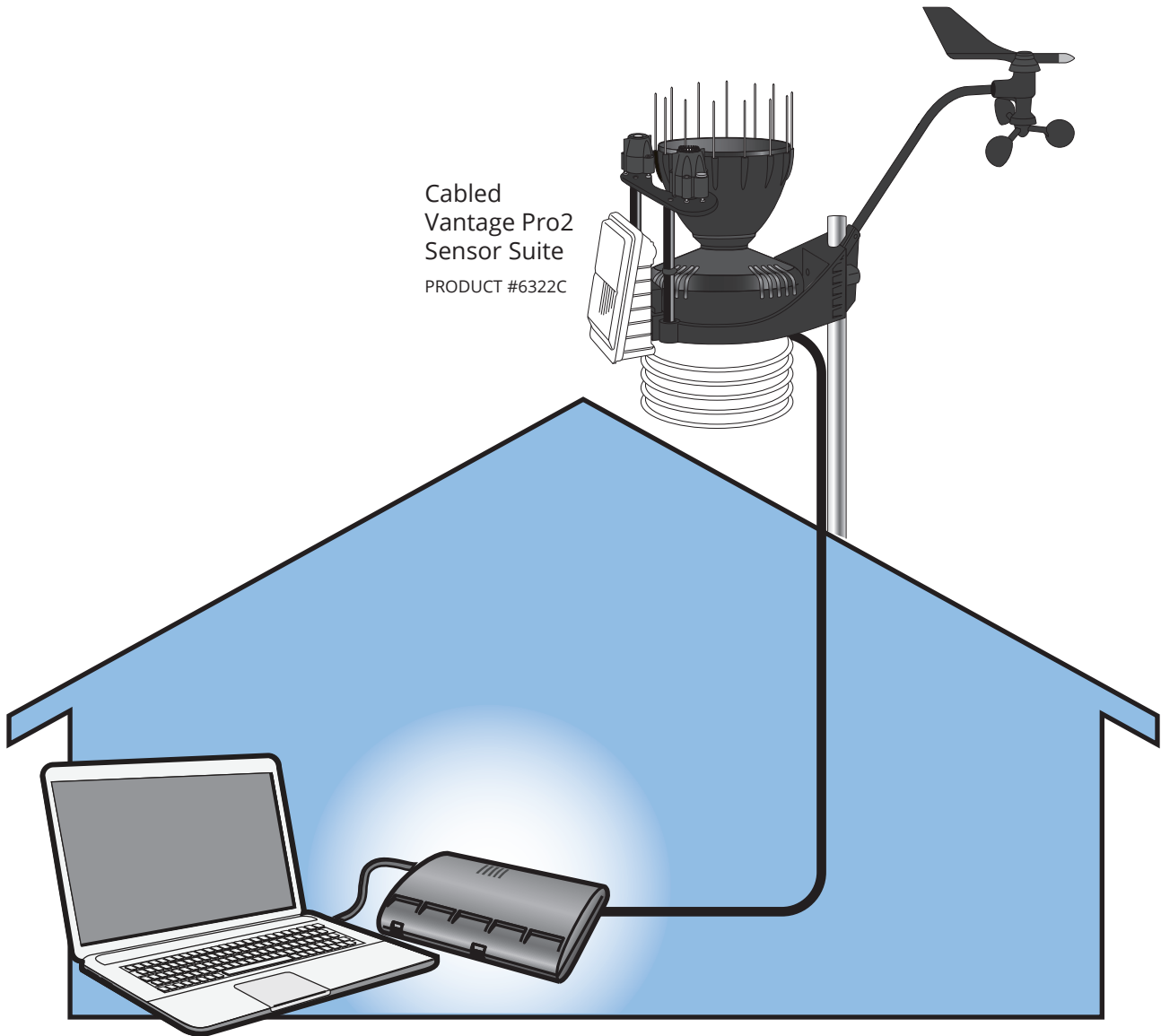
Cabled Weather Envoy PRODUCT #6316C AND WeatherLink® Data Logger PRODUCT #6510SER
