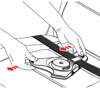
Slide the car mount forward securing the belt into the belt hook.
