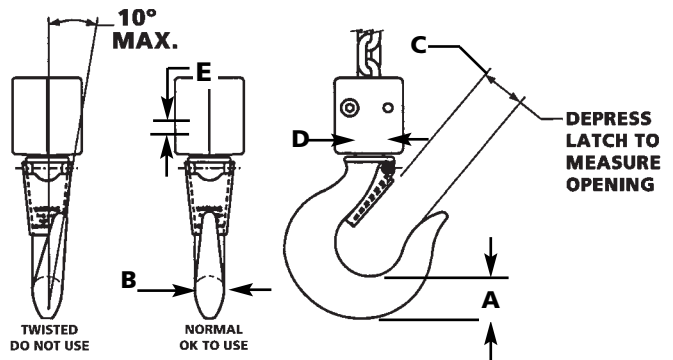
Figure 3 - Hook Inspection
