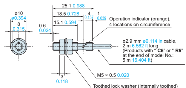
GX-305M-□ Sensor
