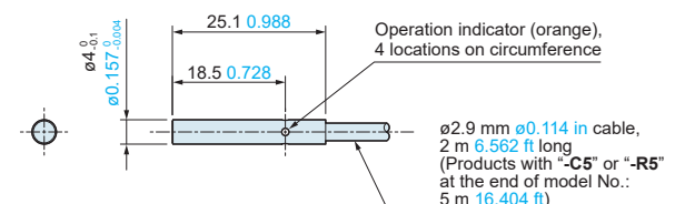
GX-305M-□ Sensor
