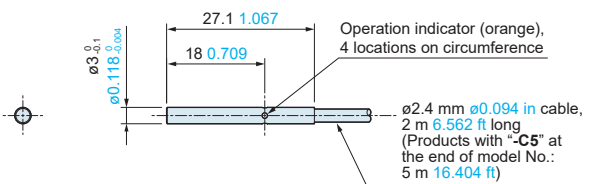
GX-305S-□ Sensor
