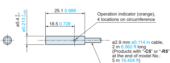
GX-305S-□ Sensor
