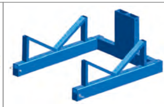
Optional Accessory(Part#3017014) ◆ Ipe Forks ◆ Load capacity - 300kg ◆ Weight - 16 kg ◆ Dimensions - 600x700x355 mm
