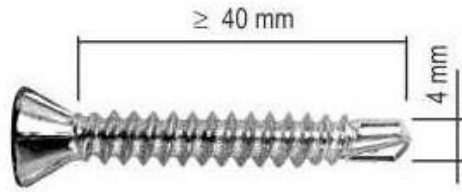
Fibercement Screw
