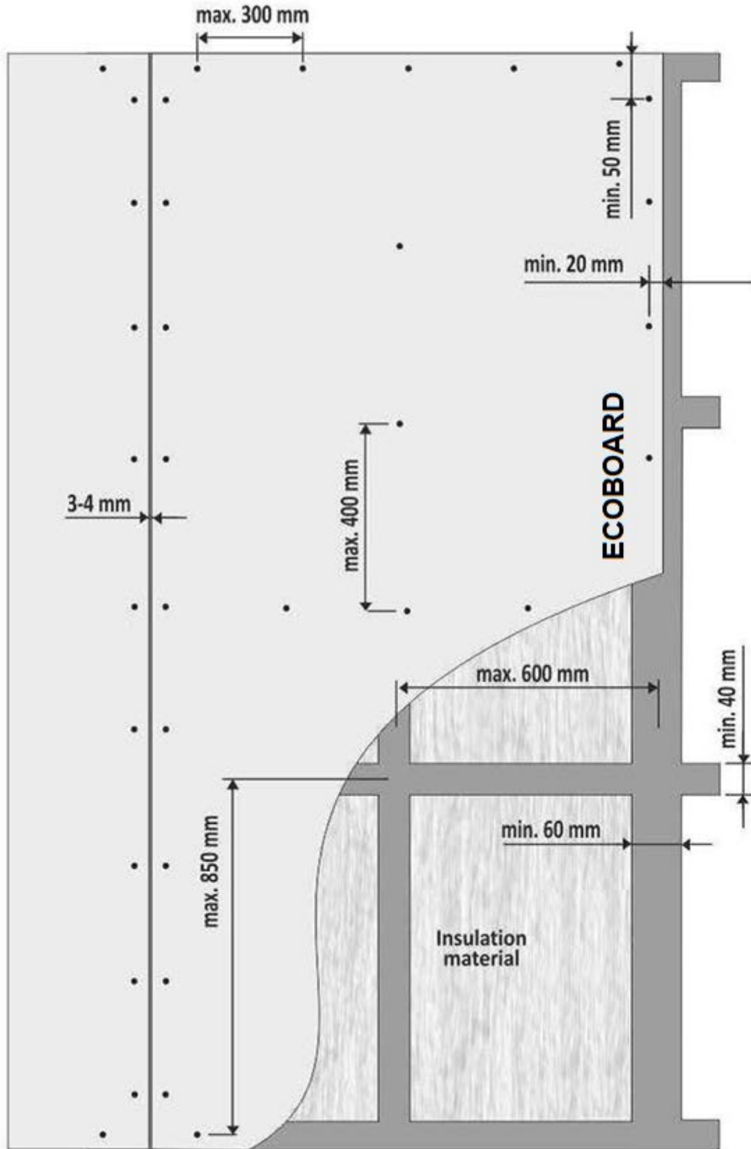
AN INSULATED WALL APPLICATION DETAIL WITH ECOBOARD
