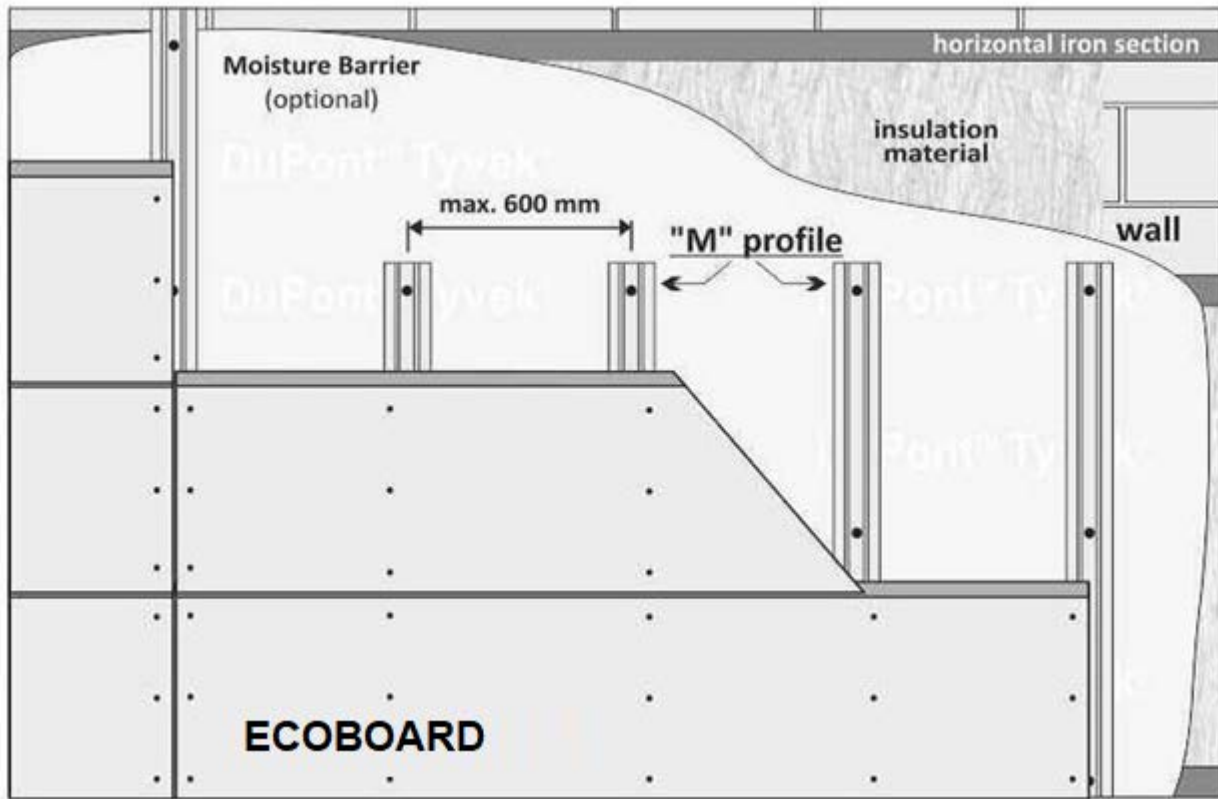
Grooved Ecoboard Application Detail
