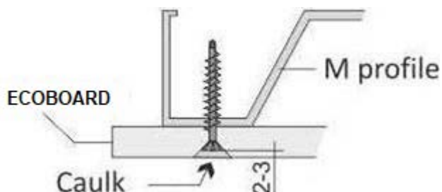
CORRECT APPLICATION
