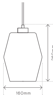
FLASK
