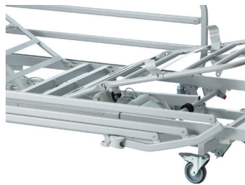
Tool-less assembly
