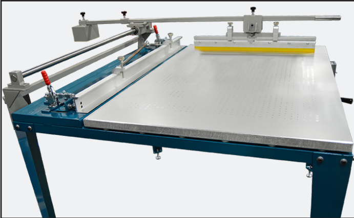
Optional Print Side Arm feature reduces operator fatigue and ensures consistent print stroke and image quality.
