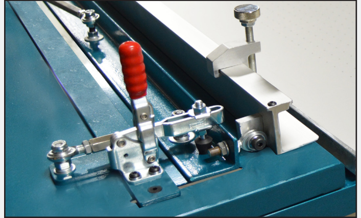
Ensure tight tolerances with the Micro Registration Lock-in feature.
