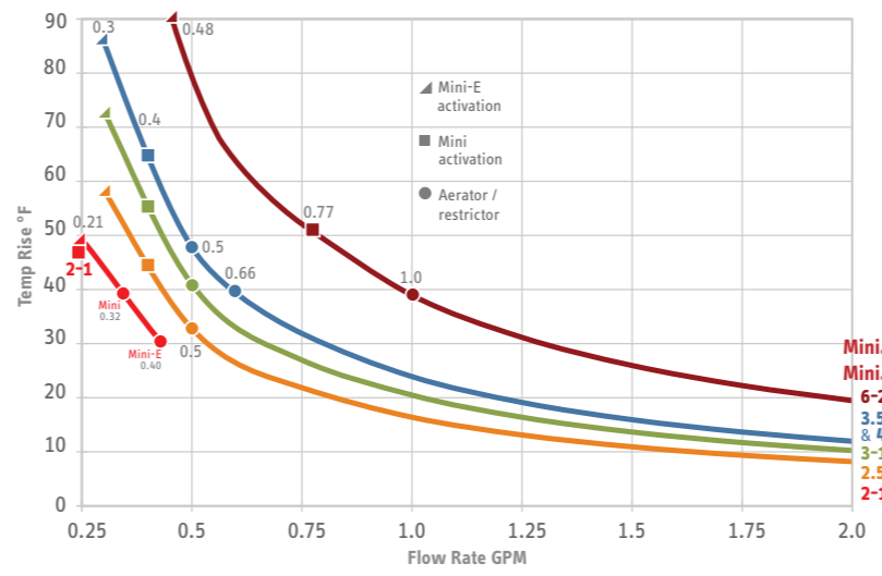
1.8 – 5.7 kW Mini./Mini-E Temperature Rise vs. Flow Rate at Max. Rated Voltage
