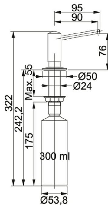
Technical Drawing
