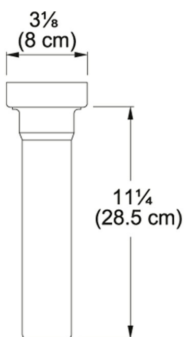
Technical Drawing
