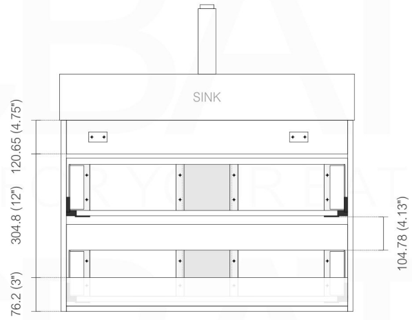
. BACK ELEVATION
