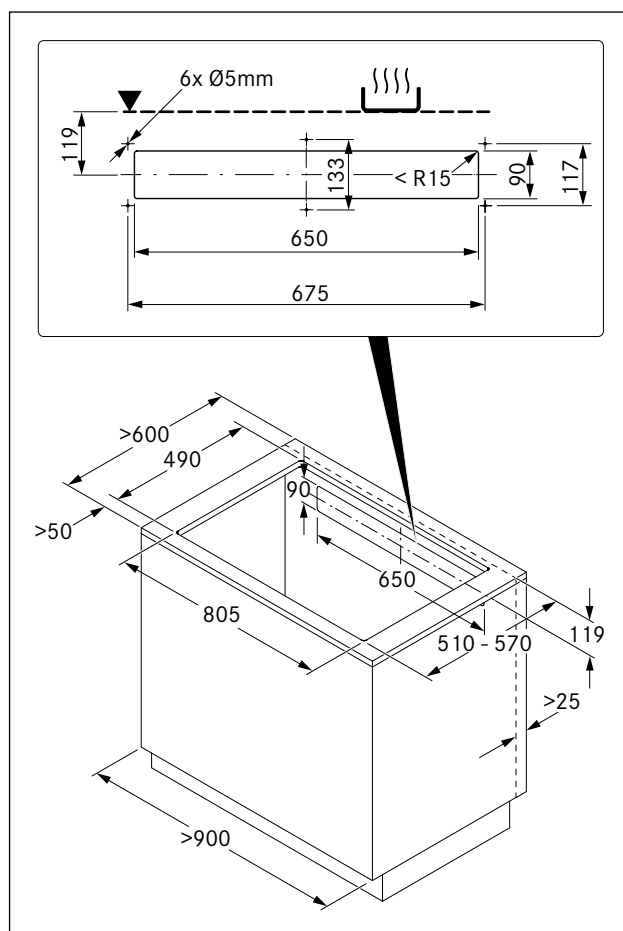
Fig. 6.9 Furniture dimensions for recirculation
