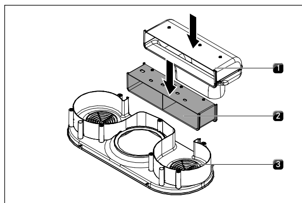
Fig. 6.29 Inserting the air duct extension
