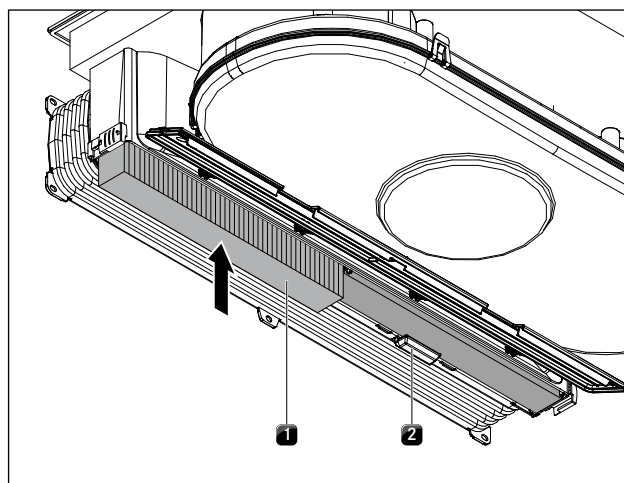
Fig. 8.9 Inserting the activated charcoal filter
