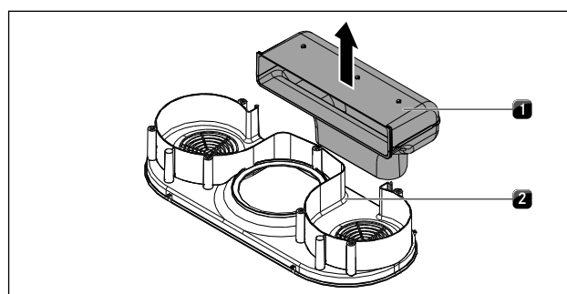
Fig. 6.28 Removing the exhaust air arc
