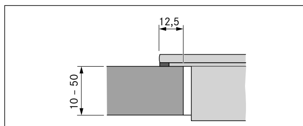
Fig. 6.6 Dimension of support for surface mounting
