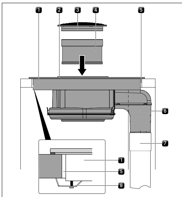
Fig. 6.35 Connect the air duct + secure
