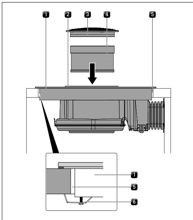
Fig. 6.17 Securing the cooktop in the middle
