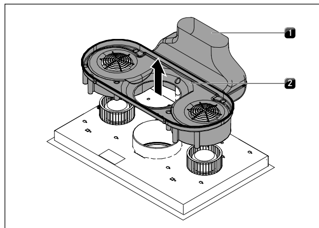
Fig. 6.27 Removing the air guiding housing
