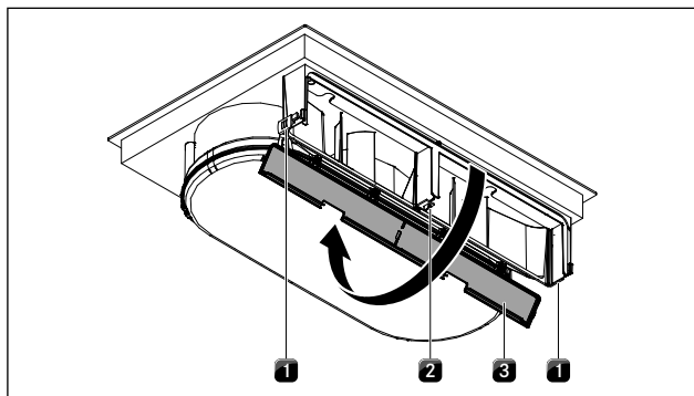
Fig. 6.14 Opening the housing cover
