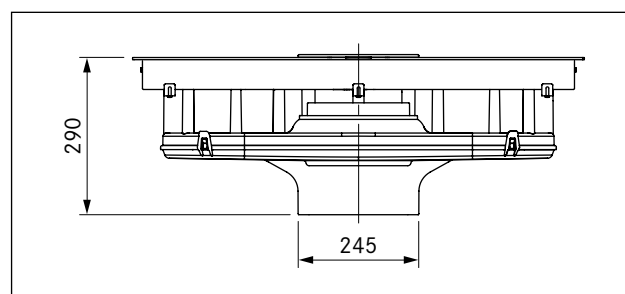
Fig. 3.2 BFIA Device dimensions front view
