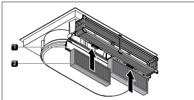
Fig. 6.16 Inserting the activated charcoal filter
