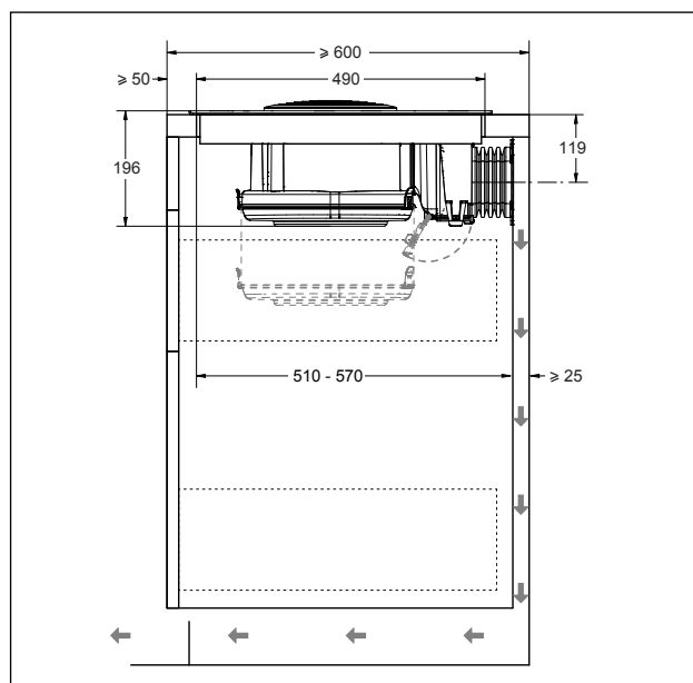
Fig. 6.10 Installation dimensions for recirculation, depth of worktop 600 mm
