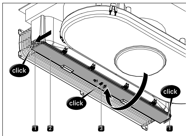
Fig. 8.10 Closing the activated charcoal filter housing cover
