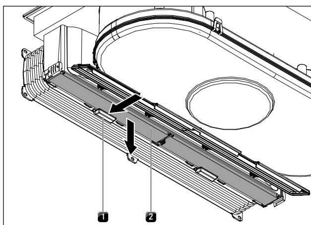
Fig. 8.8 Removing the activated charcoal filter
