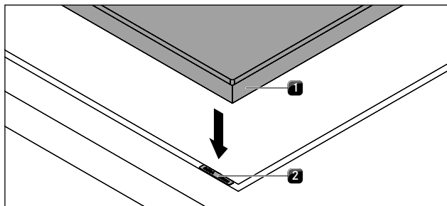
Fig. 6.34 Height adjustment plates
