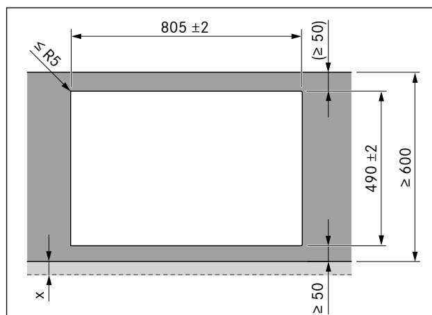
Fig. 6.5 Cut-out dimensions for surface mounting
