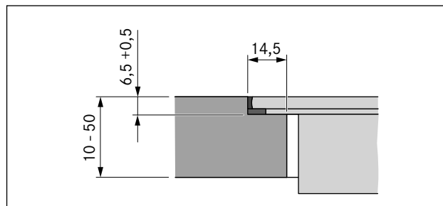
Fig. 6.4 Dimension of groove for flush installation
