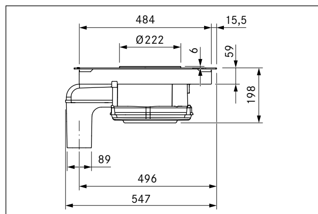
Fig. 3.3 BFIA Device dimensions side view
