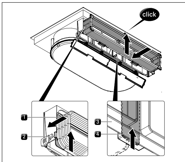
Fig. 6.15 Mounting the frame of the flexible duct
