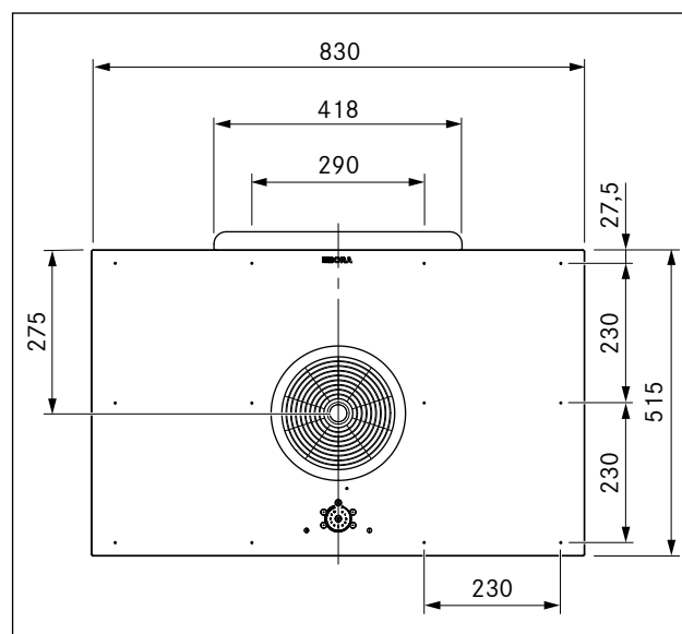
Fig. 3.1 BFIA Device dimensions aerial view
