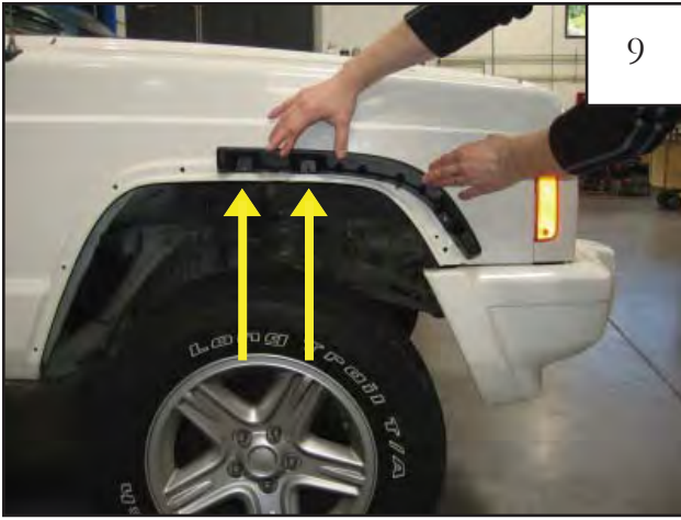
Position inner piece P1 (D1 for driver side) on fender, aligning rear two holes in the inner piece with existing factory holes in sheet metal.
