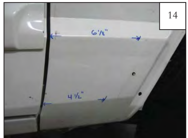
Use a grease pencil or removable marker to mark a line parallel to wheel well opening 6-1/8" from the door edge seam along style line and 4-1/2" on lower style line.
