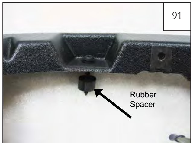
Install screw, washer, spacer combo through inner pieces P3 & P4 (D3 & D4 for driver's side) corresponding with 7/64" holes drilled in step 74. Rubber spacer should be on sheet metal side of inner piece.
