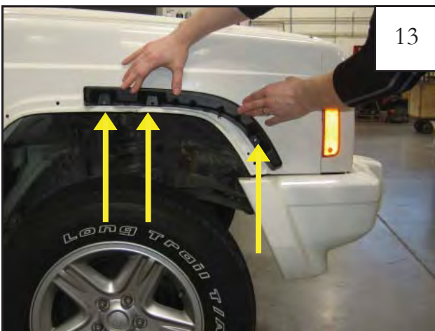
Reinstall inner piece P1 (D1 for driver side) by aligning the part with the two factory holes and newly drilled hole. Attach inner piece to the sheet metal with a screw/washer and flange nut in each hole location. Only hand tighten at this time.
