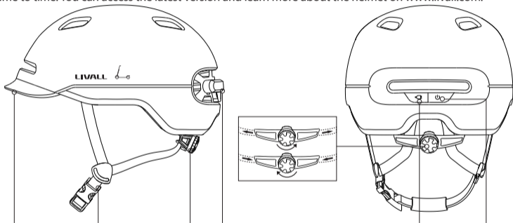
Visor Chinstrap Tension adjuster Taillight Magnetic USB charging port Power Switch
