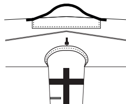
-9- Once the loop is out, Redo the knot originally present on the spectra loop in order to lock it. Reassemble your REACTOR Valve.
