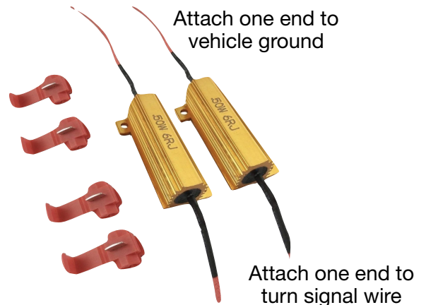
Load Resistors for Turn Signals (purchased separately)
