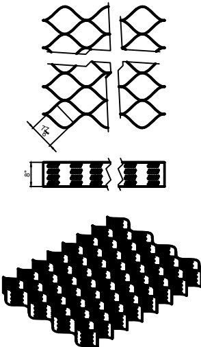
8" Geocell (art.8720)
