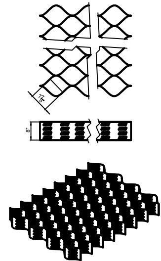
8" Geocell (art.8720)
