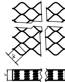
8" Geocell (art.8720)
