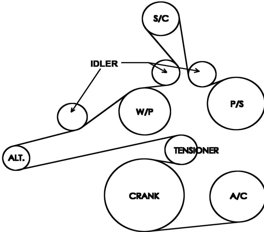
HEMI Belt Routing Diagram
