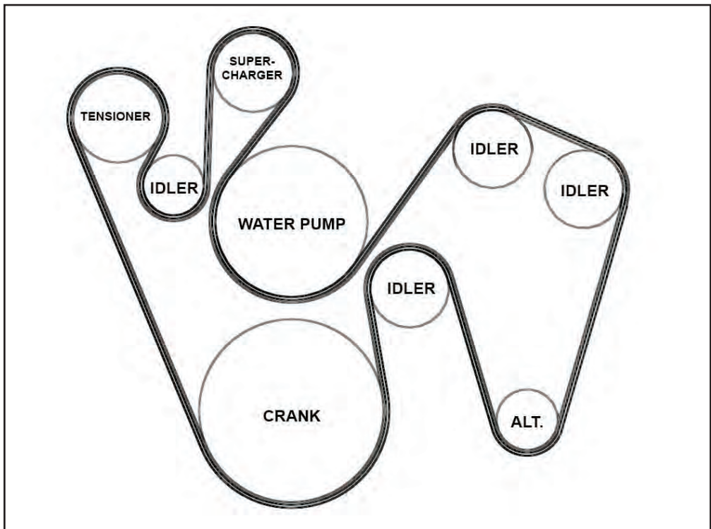
2013-2015 Belt Routing Diagram 2013-2015 = Gates# K061020 (Shorter Belt)
