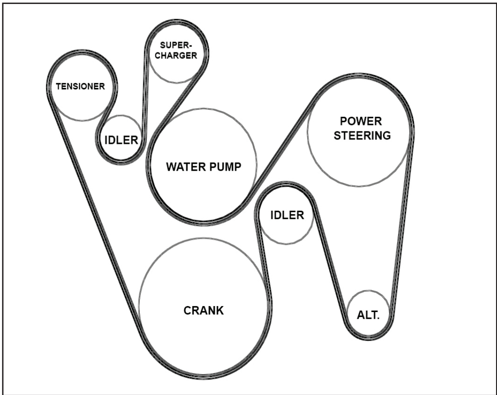
2010-2012 Belt Routing Diagram Gates# K061054 (Longer Belt)
