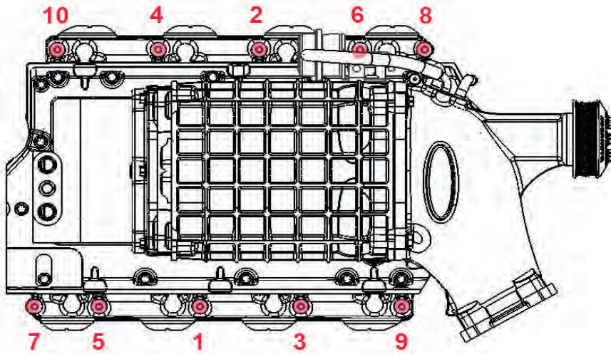
Supercharger Torque Order Diagram
