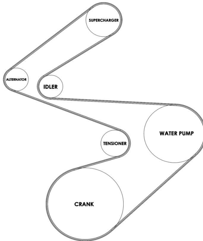
Belt Routing Diagram
