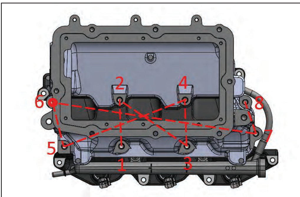
Torque Sequence for Upper Intake Manifold (18 ft-lbs)
