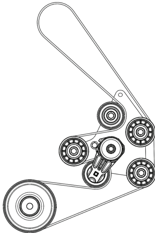
Supercharger Belt Routing Diagram (Gates#K060891)
