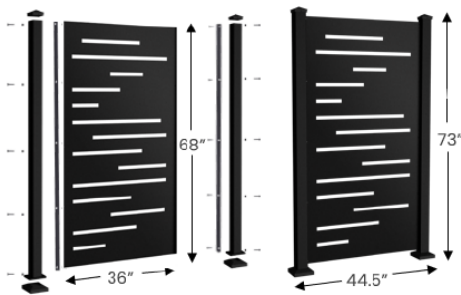
STANDARD ASSEMBLY
