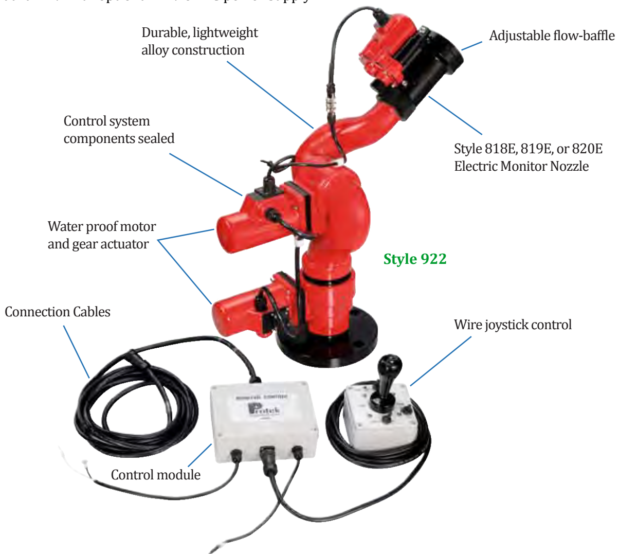
Style 922 monitor shown with standard accessories: Electric nozzle, control module, connection cables, cable joystick control
