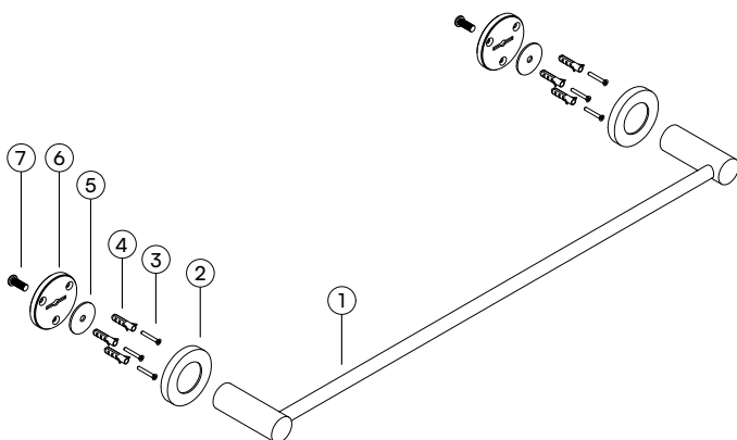
EXPLODED VIEW
