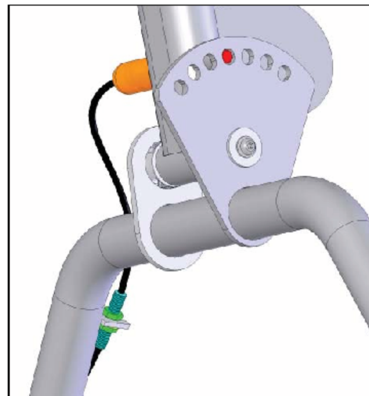
FIG. 8 This illustration depicts the ideal setting for the plunger, as shown flushed with the outside surface of the Adjustment Plate.
