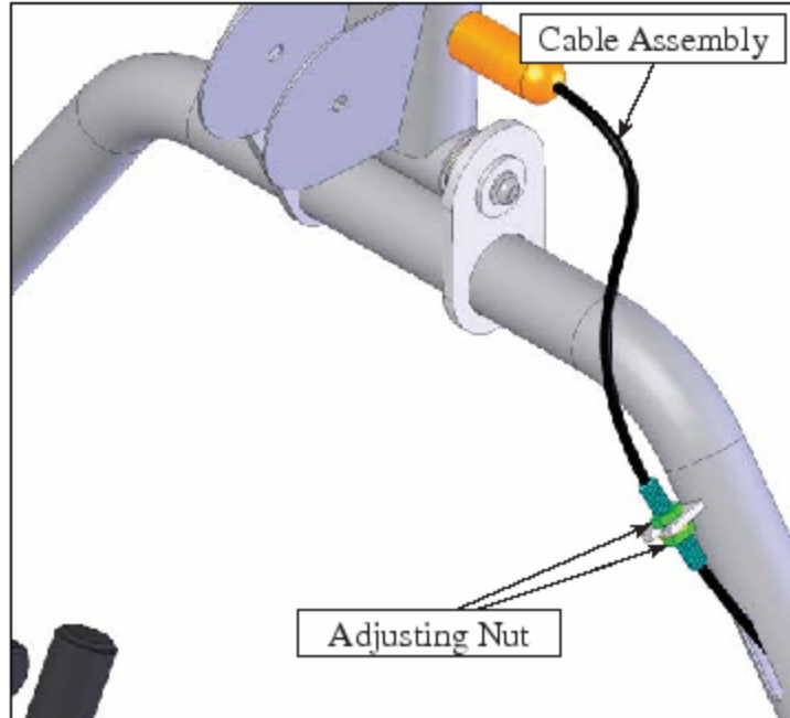
To increase or decrease the tension and play of the adjusting handle, perform the following steps: FIG. 5 Loosen the Adjusting Nuts with two 3/4 wrenches. Now tighten the top Adjusting Nut until the Handle completely disengages the Plunger from the Selector Plate. (If handle works properly go to Fig 7)
