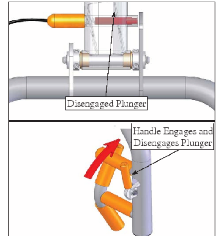
FIG. 7 Before using the machine, be sure that the Plunger fits easily into all seven (7) of the Adjustment Plate Holes and that the end of the Plunger does not make contact with the Adjustment Plate while changing from one position to the other. (if handle is loose or needs adjusting, please refer to Fig. 5 and 6.)
