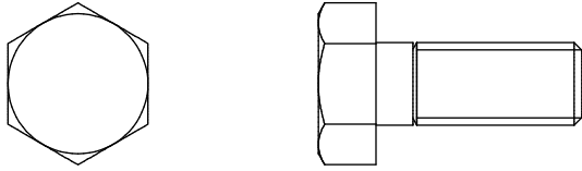
A2. M8X25L Hex Head Bolt Qty.4
