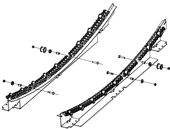
Curve Bearing Trajectory Assembly
