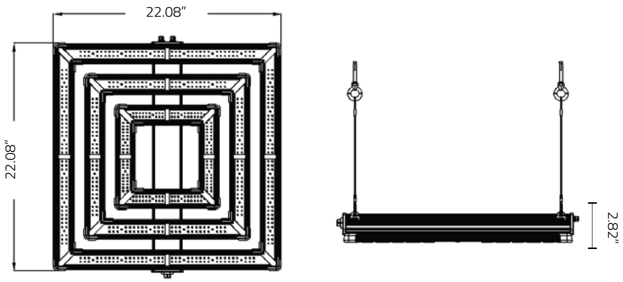
Fig1. Fixture Dimensions
