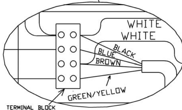
ENLARGED TERMINAL BLOCK TO CLARIFY WIRING COLOURS.
